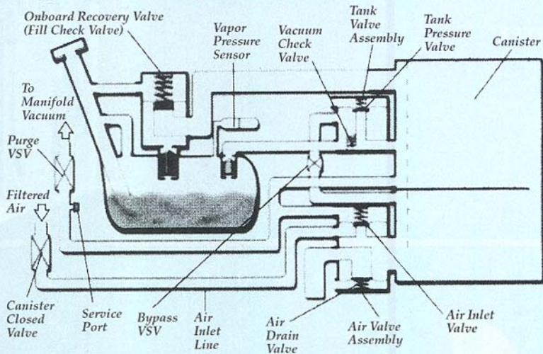
Fig. 2: Schematic of late-type (intrusive) Toyota EVAP system.
