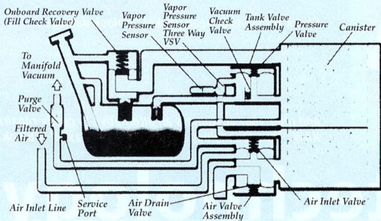
Fig. 1: Schematic of early-type (non-intrusive) Toyota EVAP system. (Diagram courtesy of Toyota Motor Co.)
